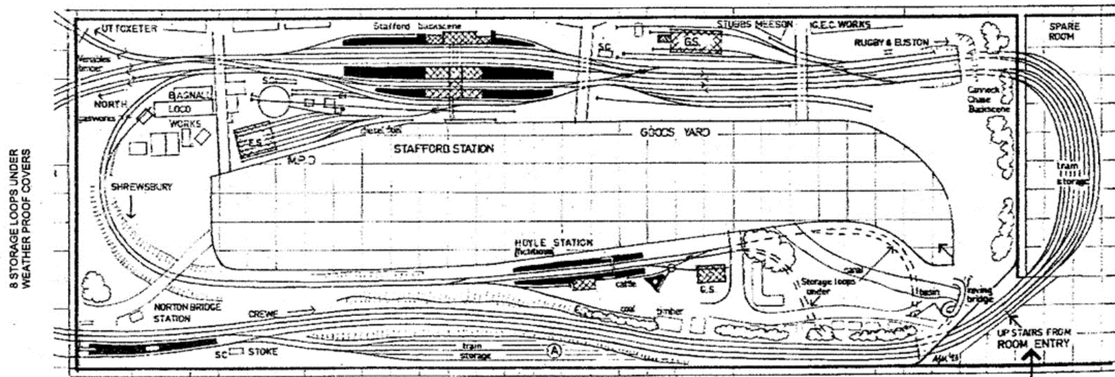
Plan: Alex Mathieson 1993. Scale: Each square represents 1 foot
